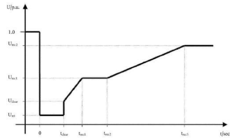
Figure X-d: Fault-ride-through profile of a Power-to-Gas Demand Unit.
