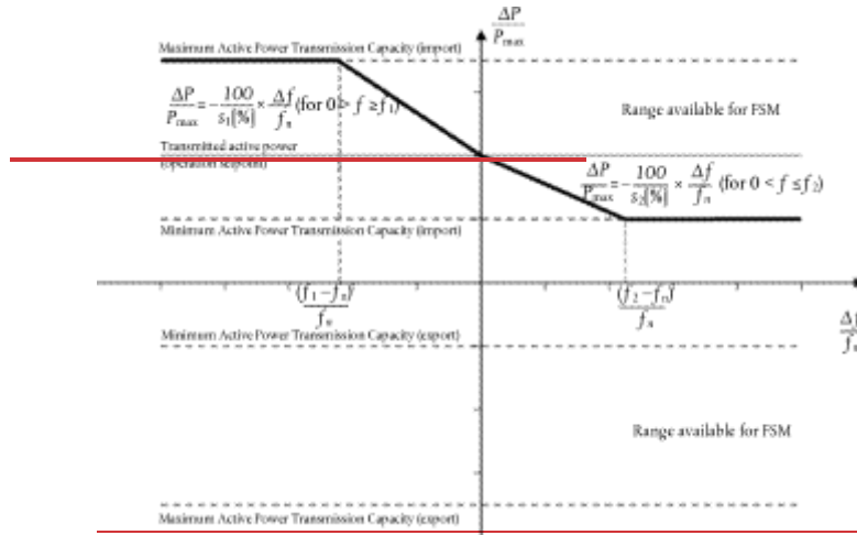
Figure 1: Active power frequency response capability of an HVDC system in FSM illustrating the case of zero deadband and insensitivity with a positive active power setpoint (import mode). In this figure, \Delta P is the change in active power output from the exchange by an HVDC system with the network at its connection point based on its actual operating point, P_{max} is maximum transmission capacity of the HVDC system, f_n is the target frequency in the AC network where the FSM service is provided, and \Delta f is the frequency deviation in the AC network where the FSM service is provided, \Delta P1 is the agreed power change for the FSM at reaching the frequency threshold value \Delta f1 , \Delta P2 is the agreed power exchange at reaching the frequency threshold value \Delta f2 , \Delta f_{db} is the deadband of the power frequency response, \Delta f_{insensitivity} is the frequency response insensitivity (or else the permissible tolerance allowed), s1 is the droop value for the given \Delta P1 and s2 is the droop for the given \Delta P2 .
