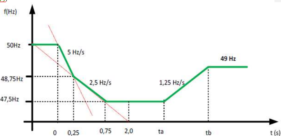
Figure X-b: The frequency ride through profile that an HVDC system should remain connected to the network for the case of under-frequency. The value t_a and t_b shall be specified by each relevant TSO, but longer than for A-PPMs according to Article 39 .
